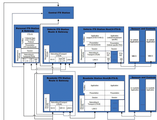
Connections between personal ITS stations and other ITS stations
